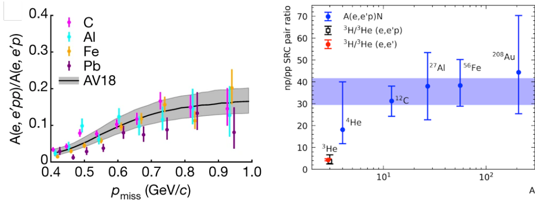
Figure 26: Left: The ratio of (e,e'pp) to (e,e'p) cross sections for different nuclei as a function of the missing momentum of the first proton [631]. The gray band shows a factorized calculation for carbon (C) using the Generalized Contact Formalism (GCF) and the AV18 potential. Right: Extracted np -SRC/ pp -SRC ratio from recent comparisons of ^3\text{H} and ^3\text{He} scattering along with previous world's extractions [632].
